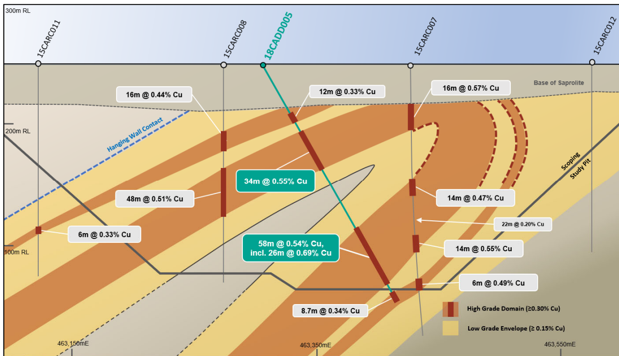
Figure 2: Cross Section through the Bindi Hinge Zone (6574300mN).
