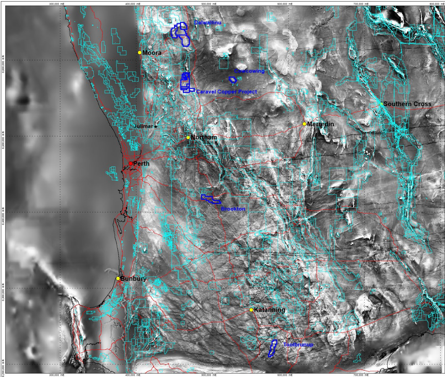
Diagram 1: New Caravel project locations overlay aeromagnetic image
